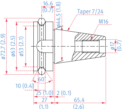
MAS 403 BT40
