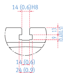
Detail B (1:2)
